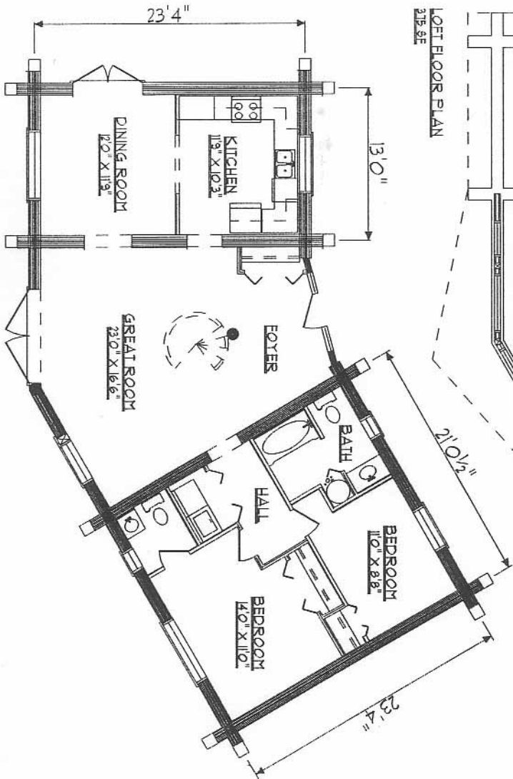
MAIN FLOOR PLAN 302 SF
