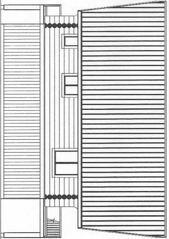
LEFT ELEVATION
