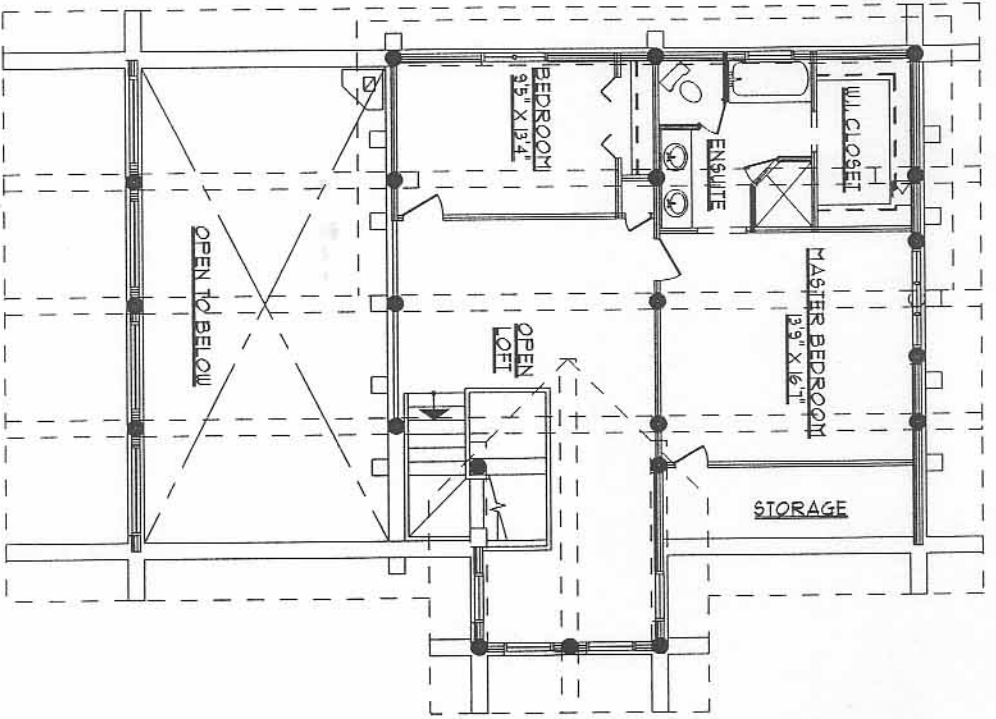
LOFT FLOOR PLAN 1060 SF
