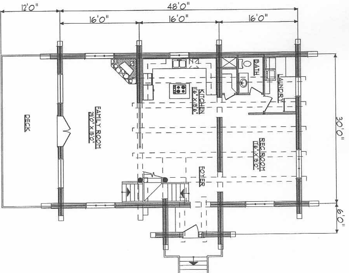
MAIN FLOOR PLAN 1556 SF
