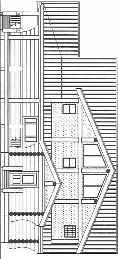
REAR ELEVATION
