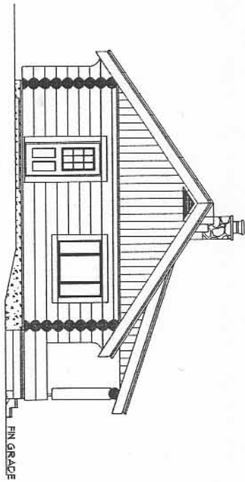
LEFT ELEVATION
